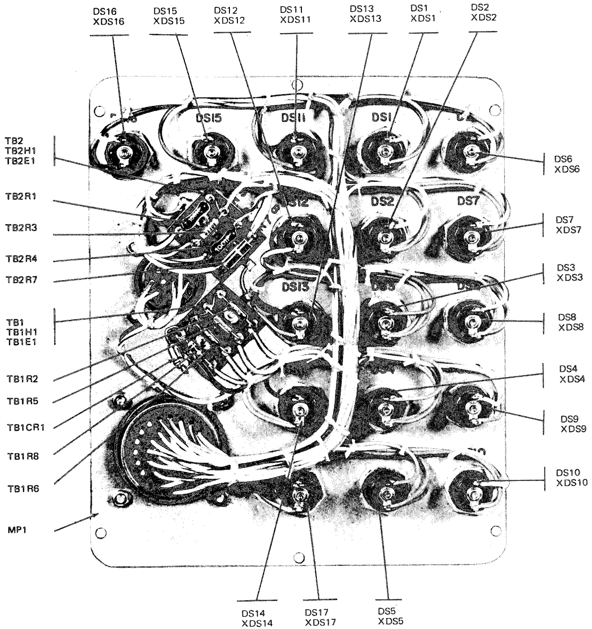
ASSEMBLY MP2A1A1 FIGURE 12
