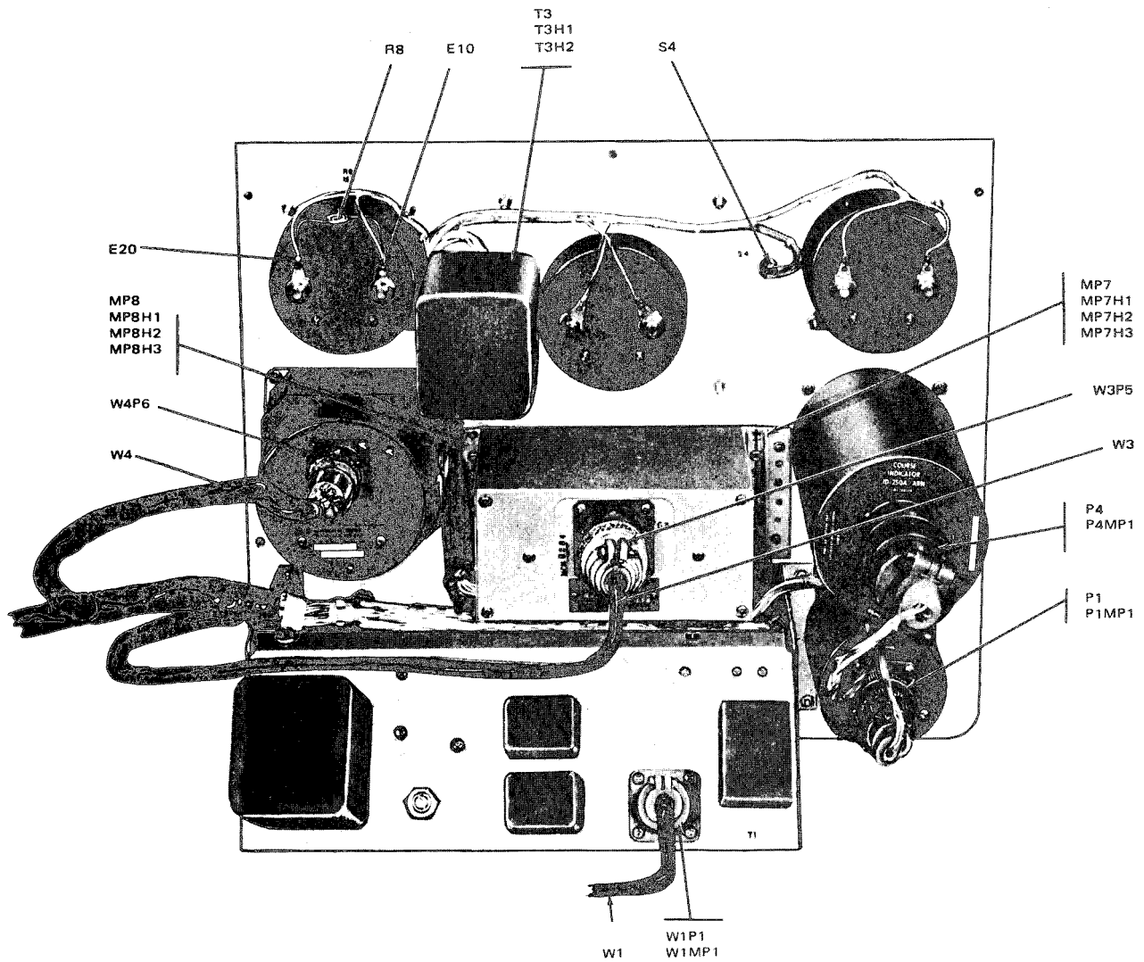
ASSEMBLY A1 FIGURE 6
