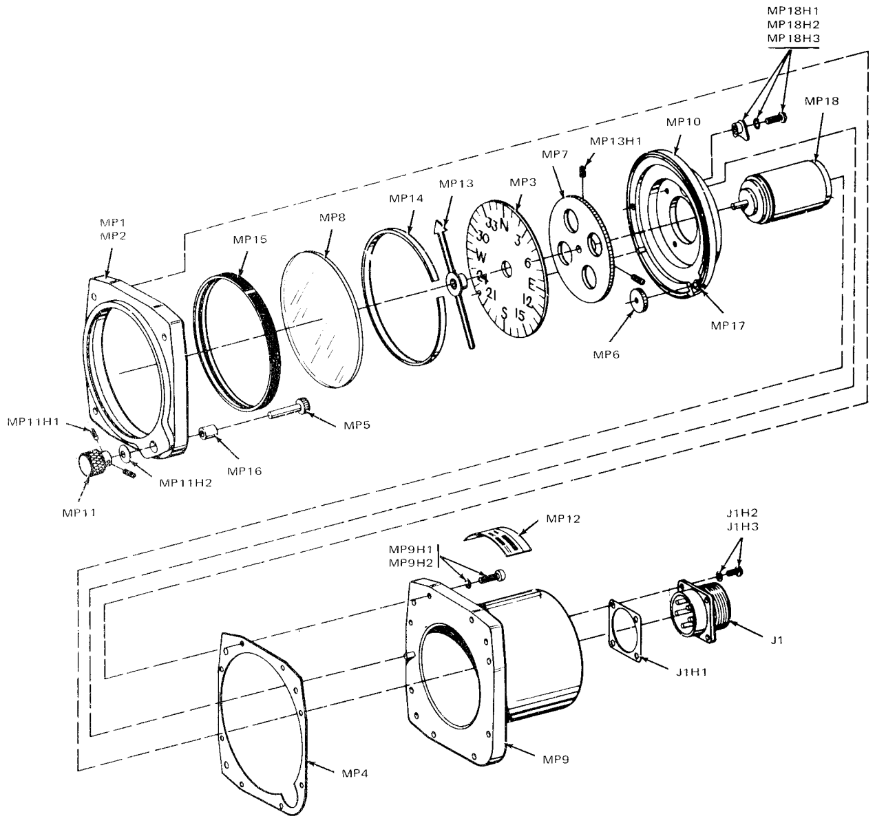
ASSEMBLY A1DS4 FIGURE 9
