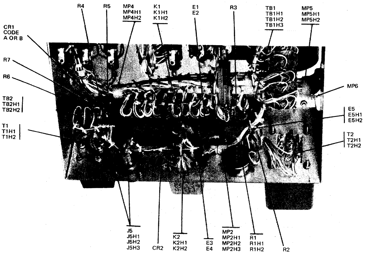
ASSEMBLY A1A1 FIGURE 5
